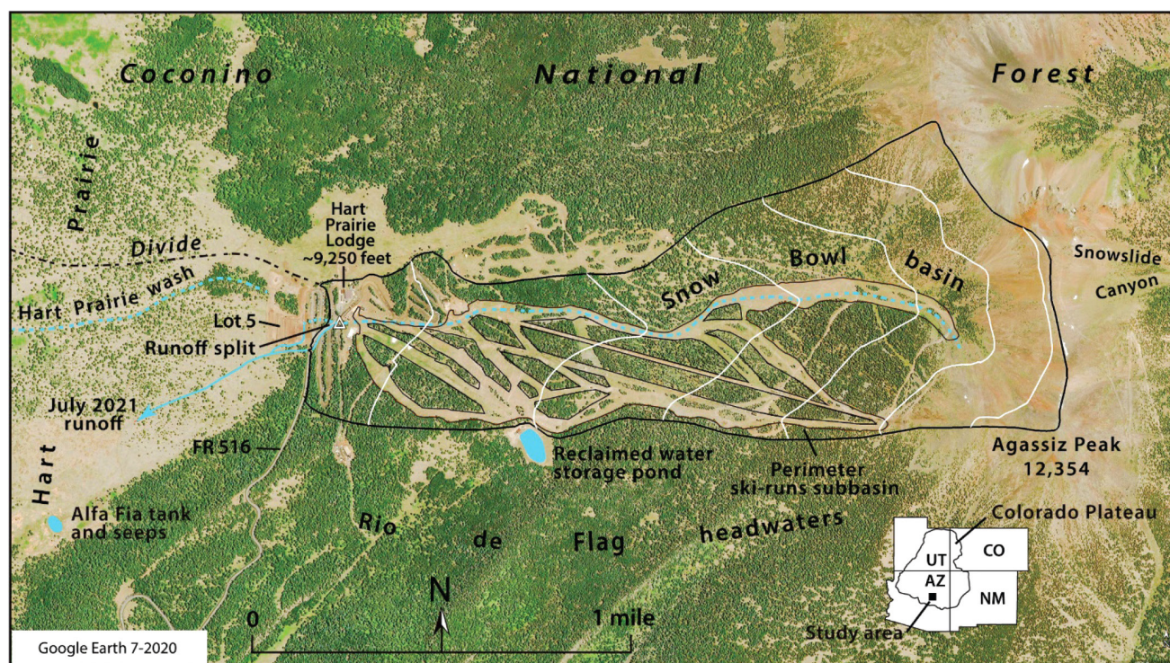
FIGURE 1 West-central side of San Francisco Mountain showing Snow Bowl drainage basin, Hart Prairie, and perimeter of 220-acre 60 percent deforested ski-runs subbasin. Contour interval 500 ft from 9,500 to 12,000 ft. Inset map showing San Francisco Mountain on southwest Colorado Plateau.
