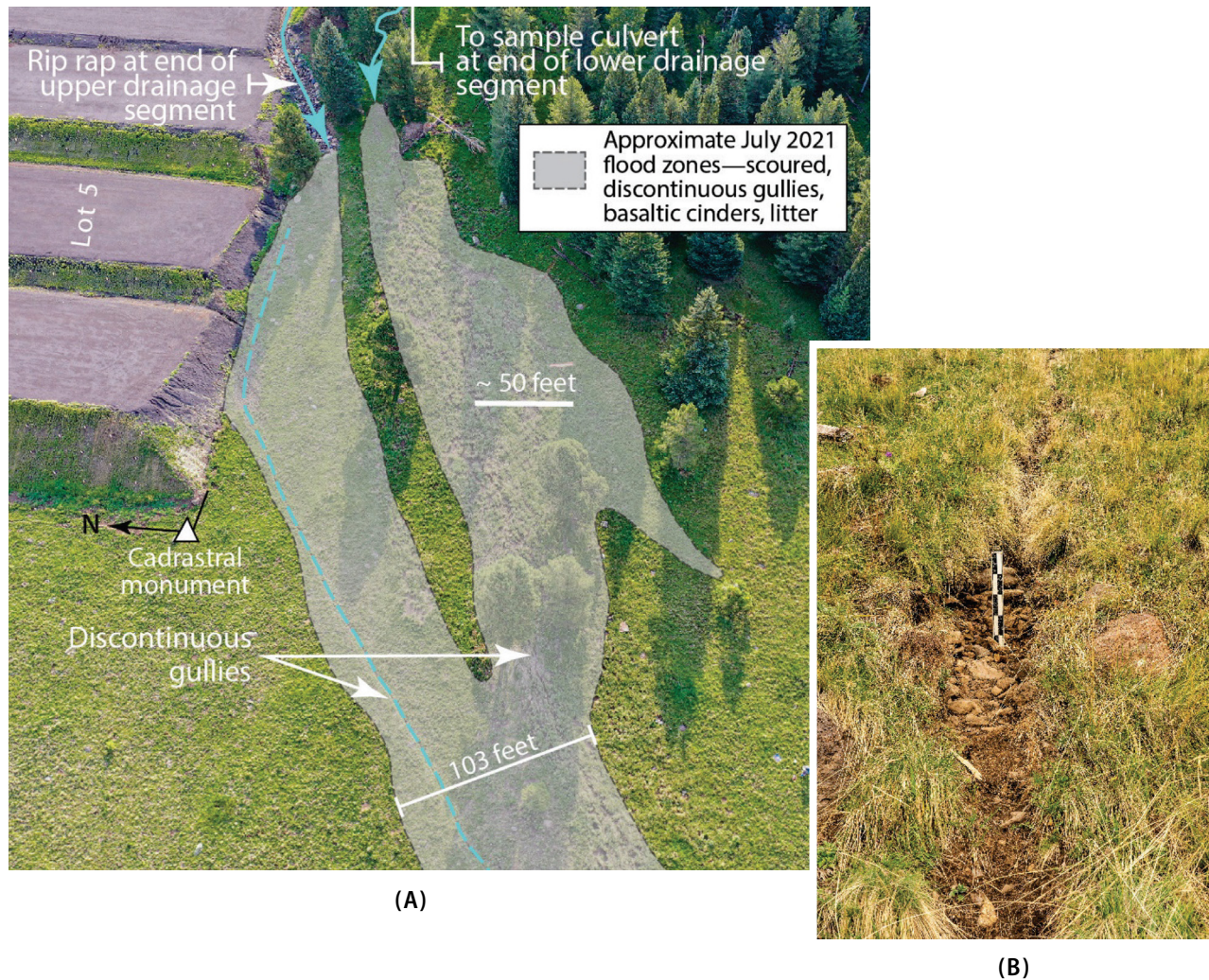
FIGURE 7 Flood zone and gullying on Hart Prairie related to runoff in late July 2021 and July 29 and August 14 of 2022, respectively. (A) Aerial view of late July 2021 runoff zone flowing from upper and lower segments of drainage system merging downstream into a single flow that extended nearly one-half mile southwest down the prairie. (B) Discontinuous gully in 2022 developing in a former foot or horse trail (scale 50 cm). Gully is two ft deep.
